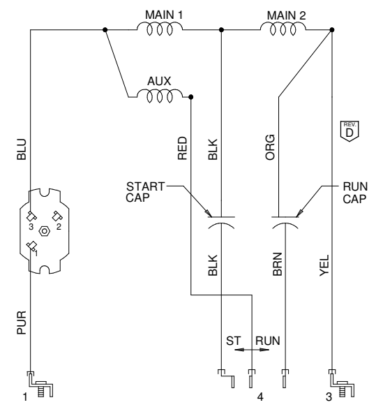
CONNECTIONS LINE 1-1 LINE 2-3
